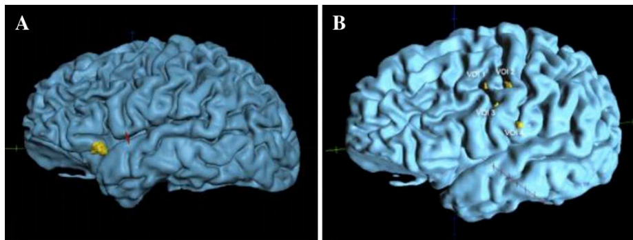
FIGURE 9. Volumetric reconstruction of axially acquired 3D T1-weighted sequences with blood-oxygen level-dependent imaging clusters shown to be significantly different in Instructor baseline vs. post-exposure (A) and in Instructor post-exposure vs. Student post-exposure (B) superimposed in yellow. Frame A demonstrates a single significantly different cluster in Brodmann area 47 [random effects GLM: t_{(7)} \geq 4.00 or \leq -4.00 , p \leq 0.005 ]. Frame B demonstrates 4 significantly different clusters, with 2 centered in Brodmann area 3, 1 in Brodmann area 7, and another in Brodmann area 40.
